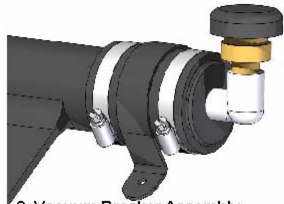
8. Vacuum Breaker Assembly
